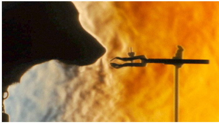
Schlierenphotographie of dog smelling, Image: Courtesy G. Settles
